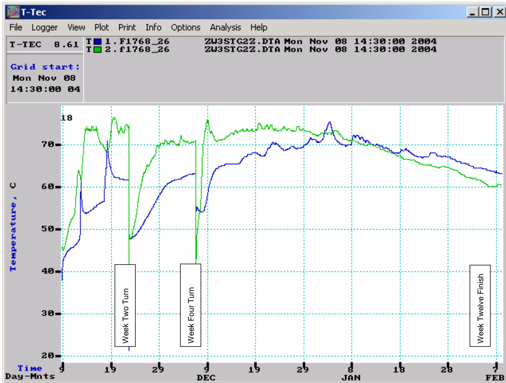
ZWSA 03 – Temperature Profile for Composting of Biodegradable Catering Products (Blue Line – Tray Temp & Green Line – Top Temp)
